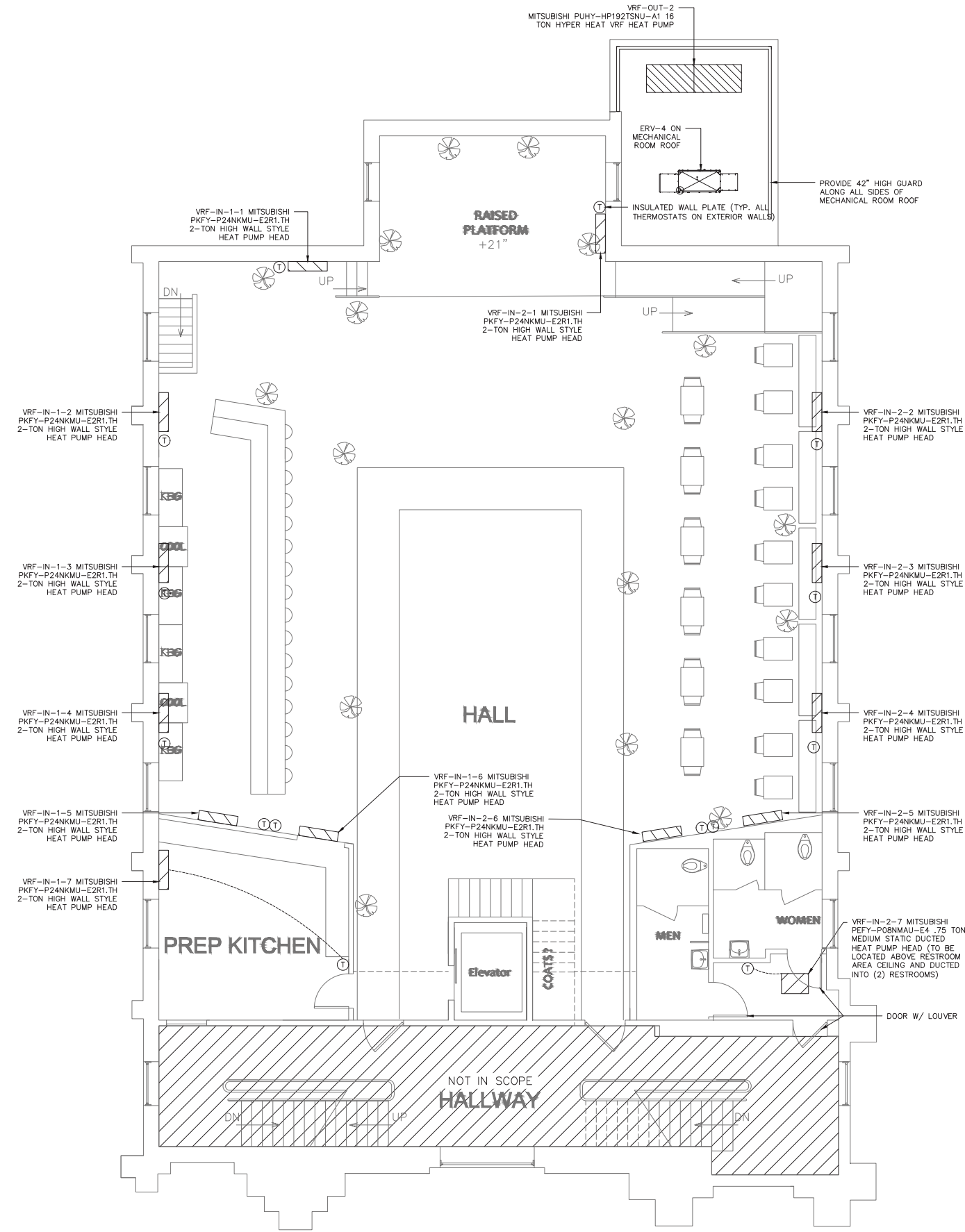
2 MAIN LEVEL HVAC PLAN - H/AC OPTION #3 3/16"=1'-0"
