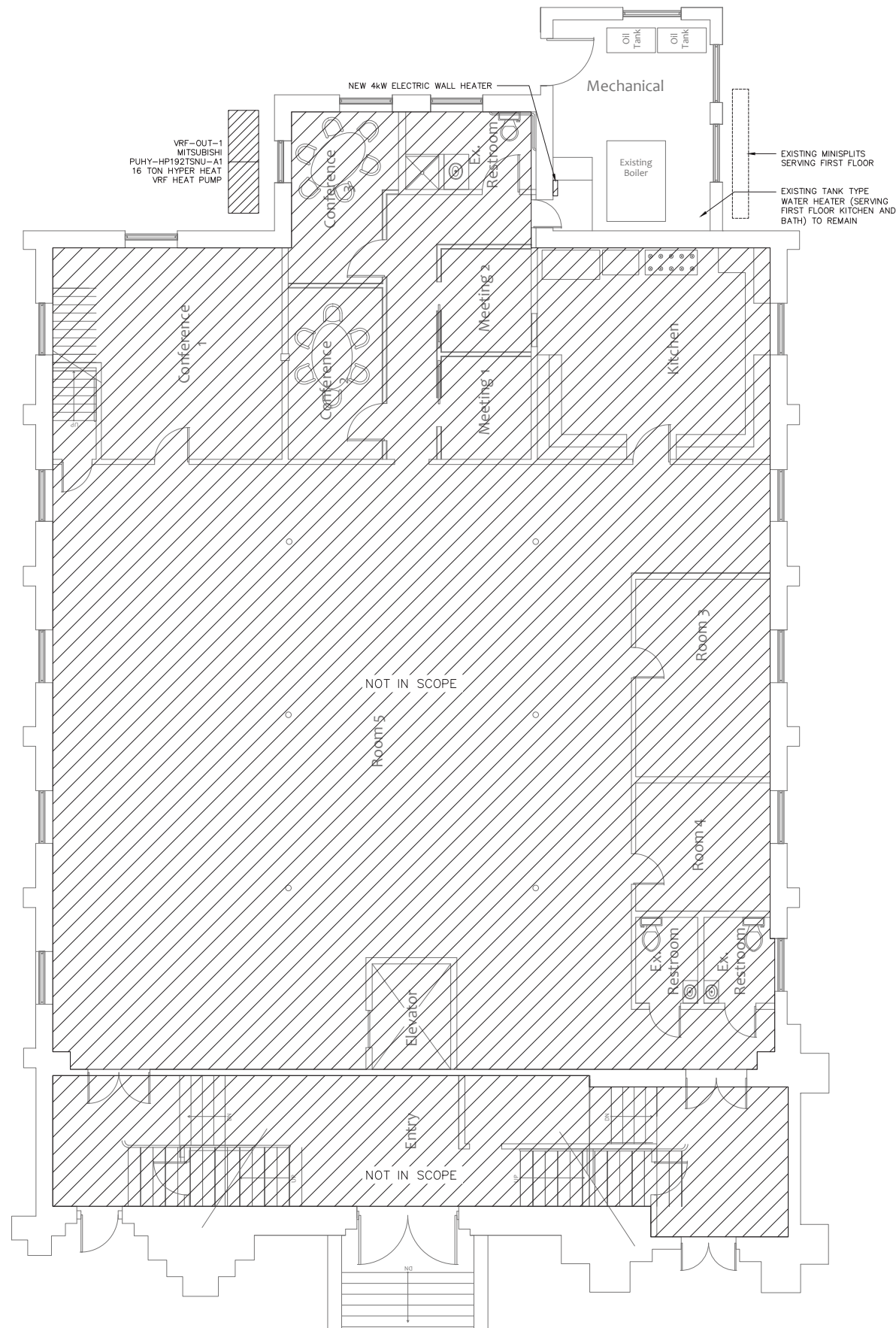
1 LOWER LEVEL HVAC PLAN - H/AC OPTION #3 3/16"=1'-0"
