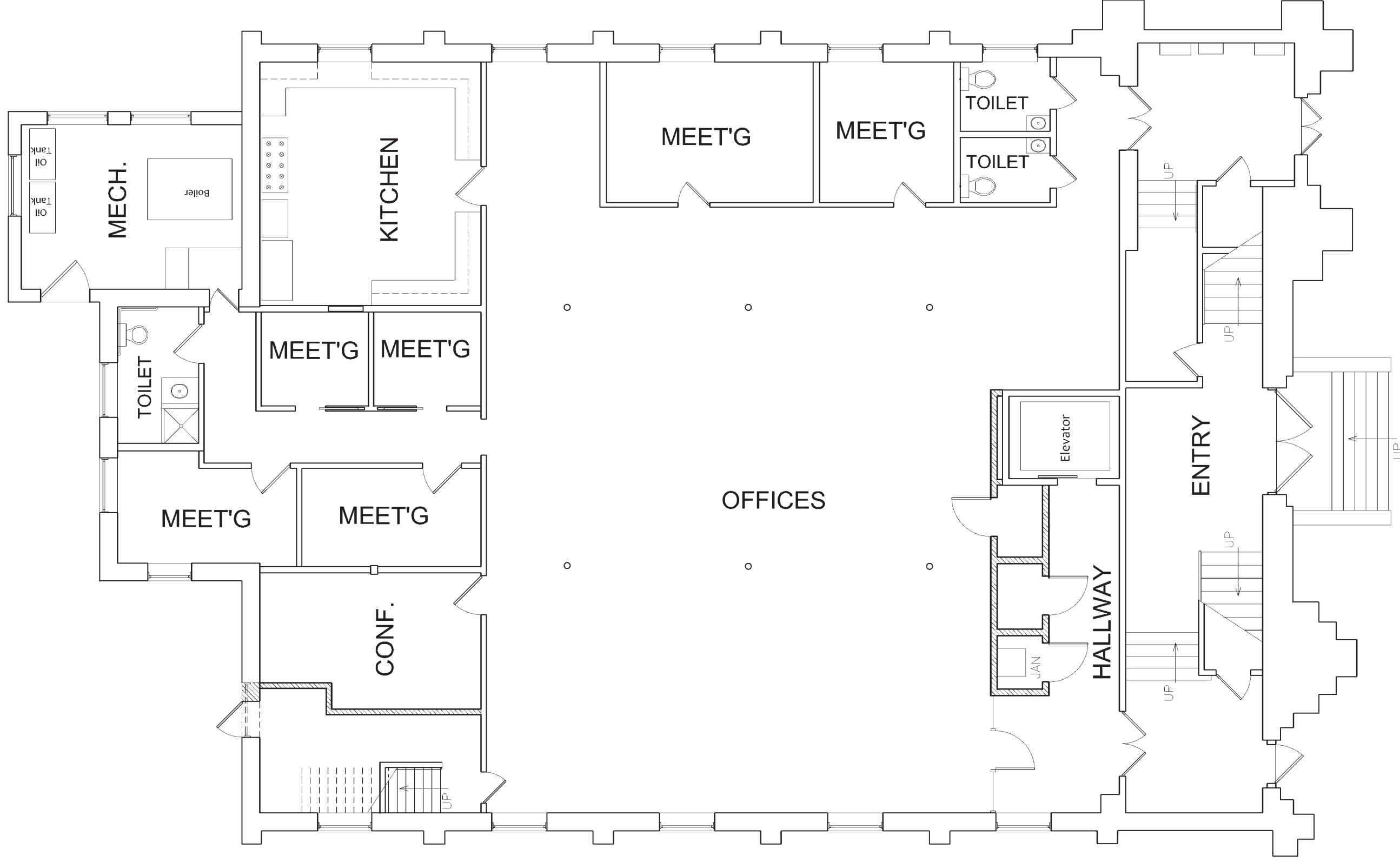
GROUND LEVEL FLOOR PLAN 1/8" = 1'-0"
