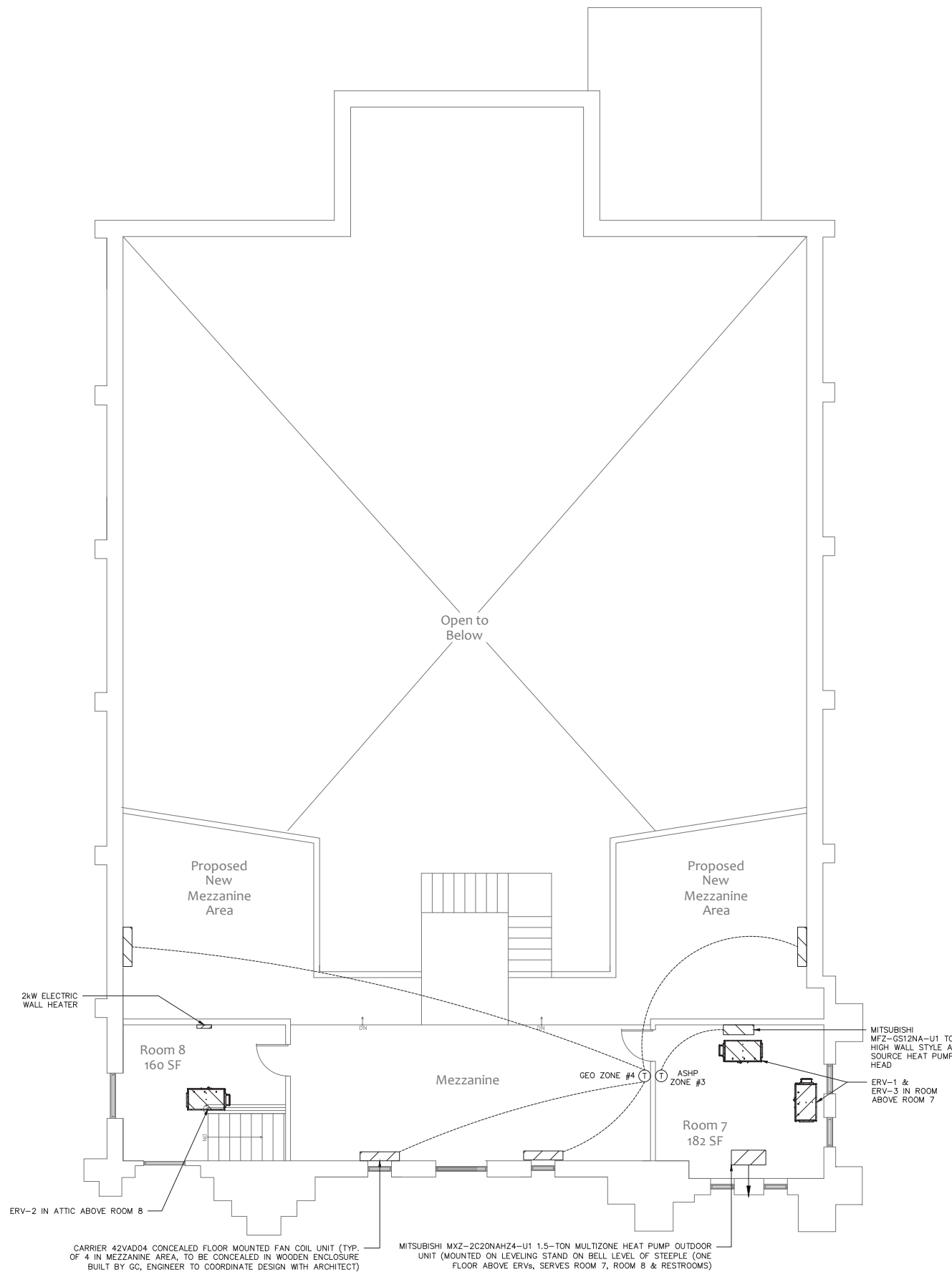
1 H1.01A MEZZANINE LEVEL HVAC PLAN - H/AC OPTION #1 3/16"=1'-0"
