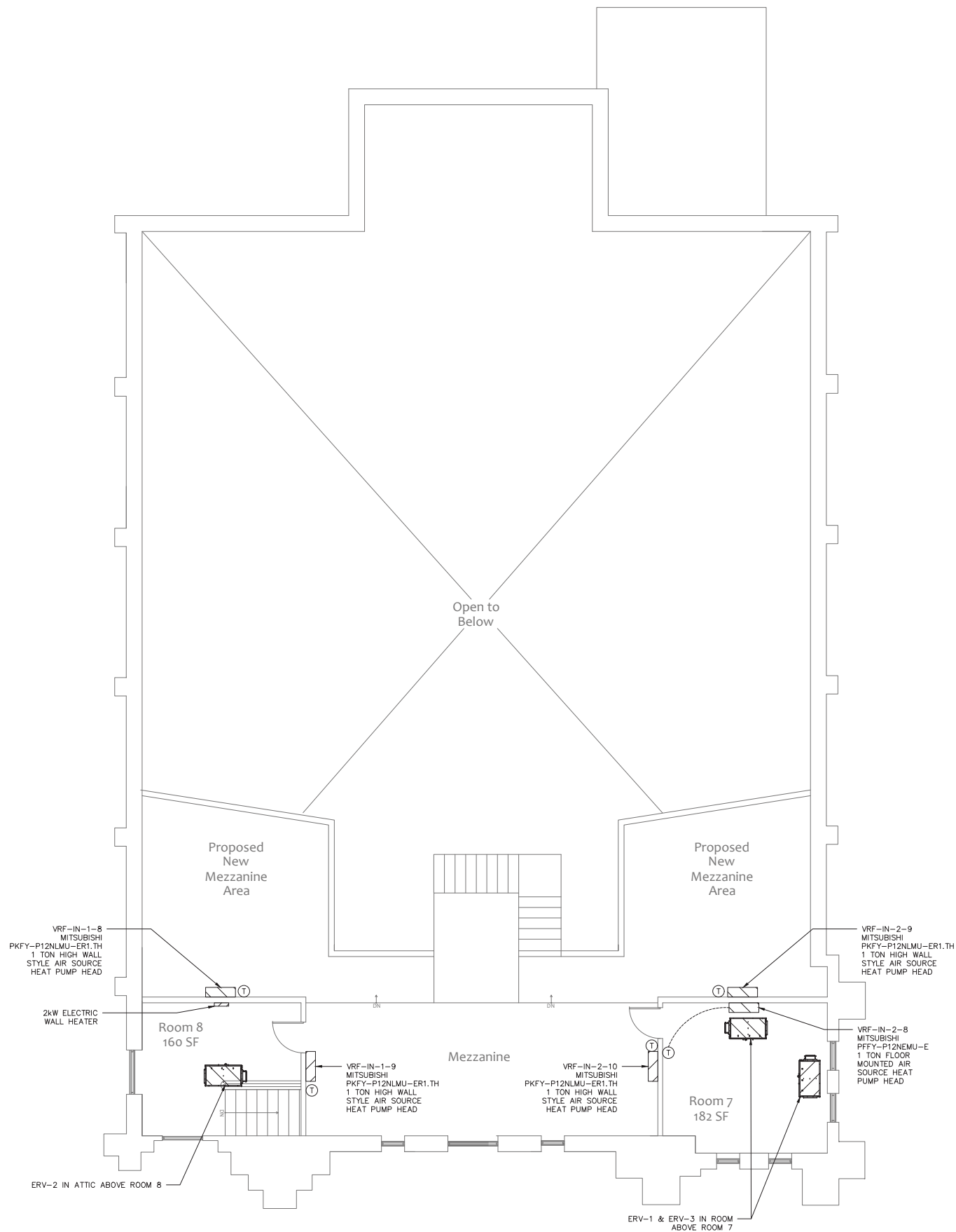
1 H1.01C MEZZANINE LEVEL HVAC PLAN - H/AC OPTION #3 3/16"=1'-0"
